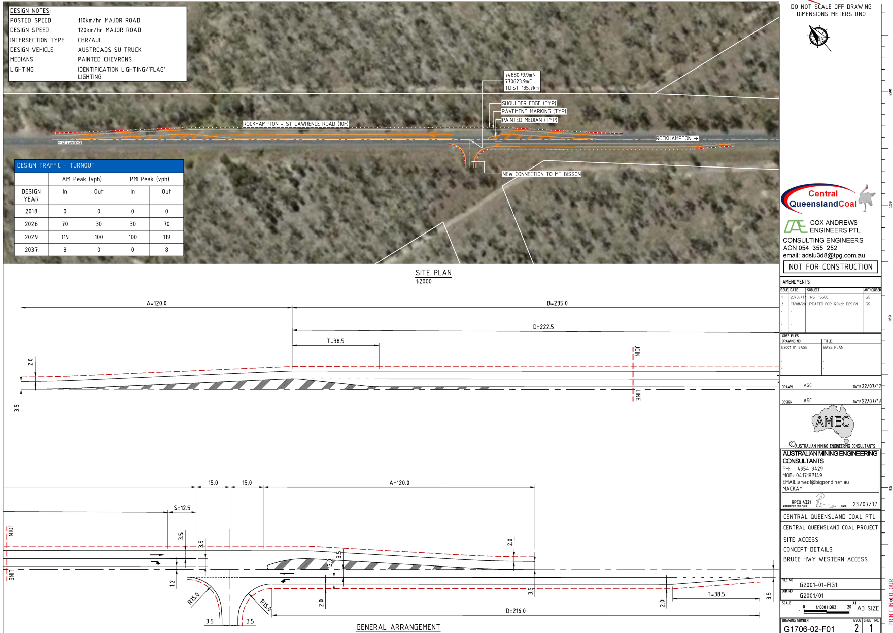
Figure 6-3: Indicative site access concept details Bruce Highway western access
