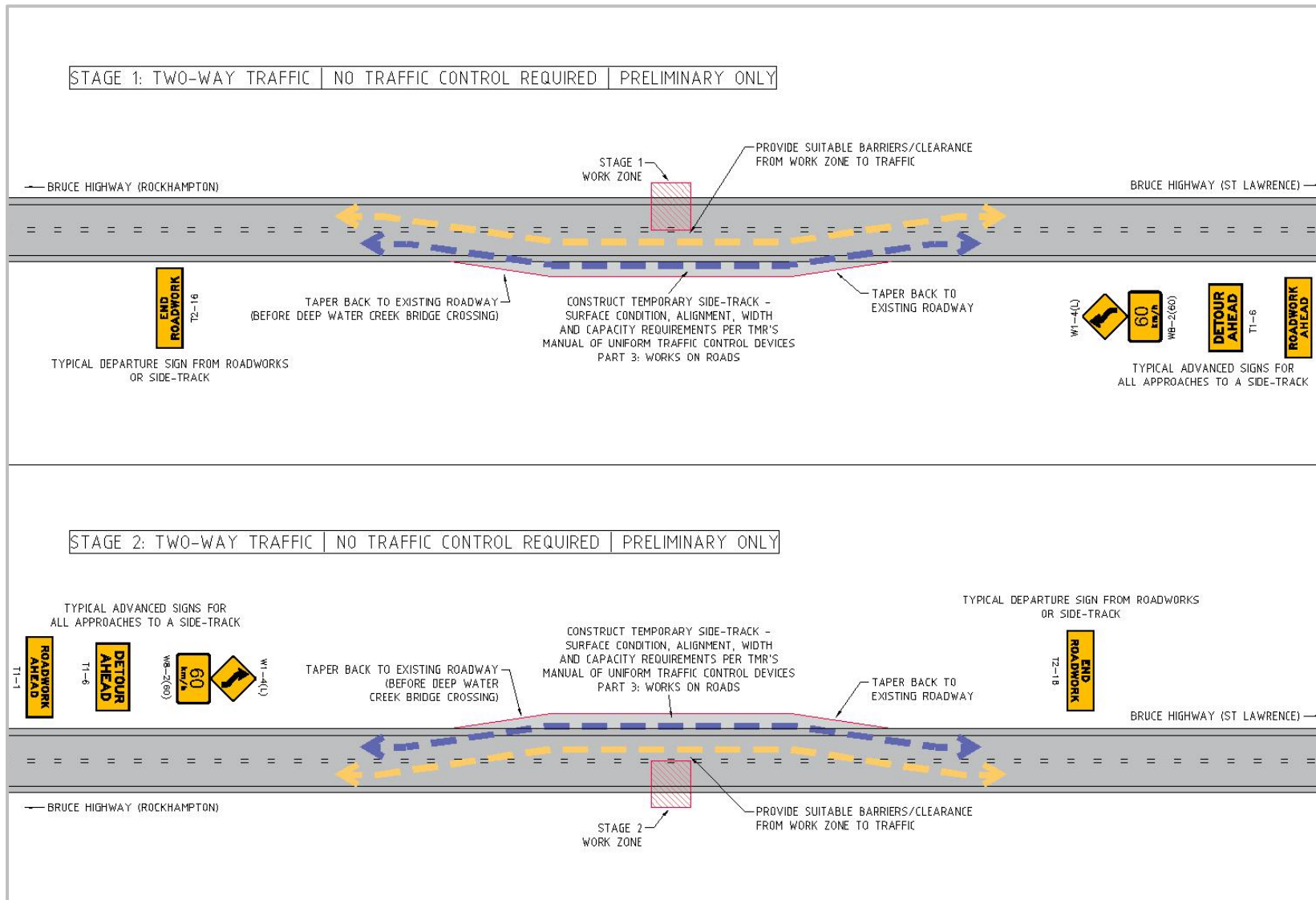
Figure 6-5 Concept traffic management methodology
