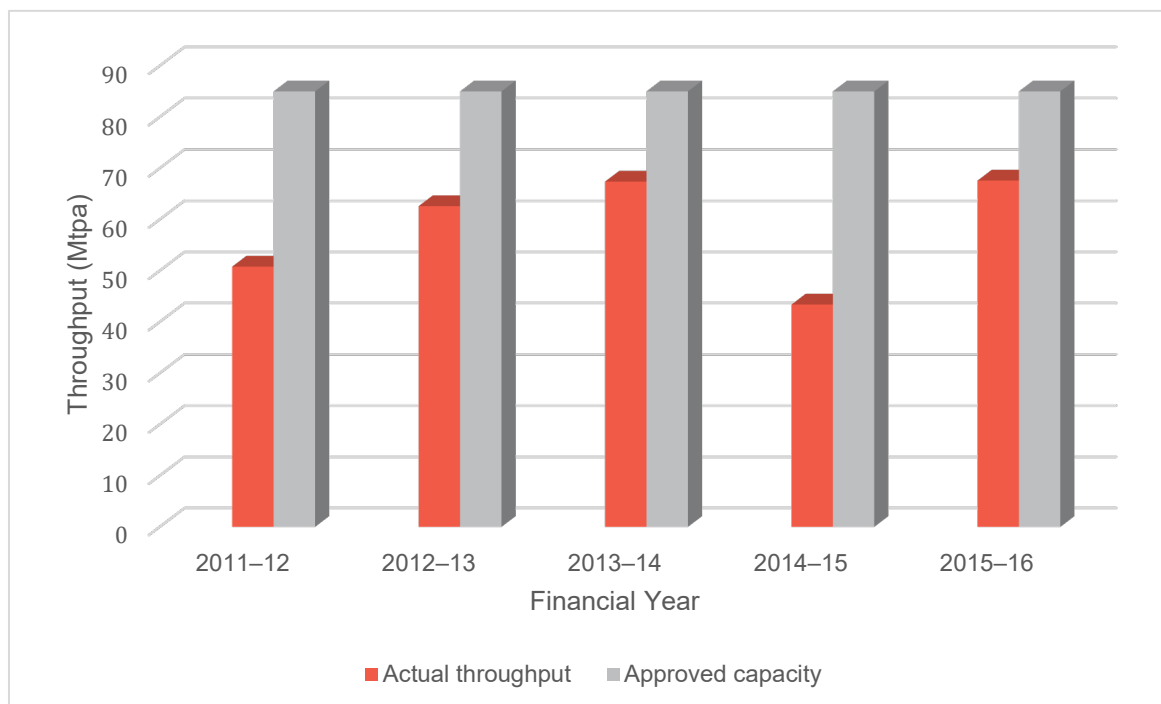
Figure 6-10: DBCT's actual throughput and approved capacity from 2011 to 2016
