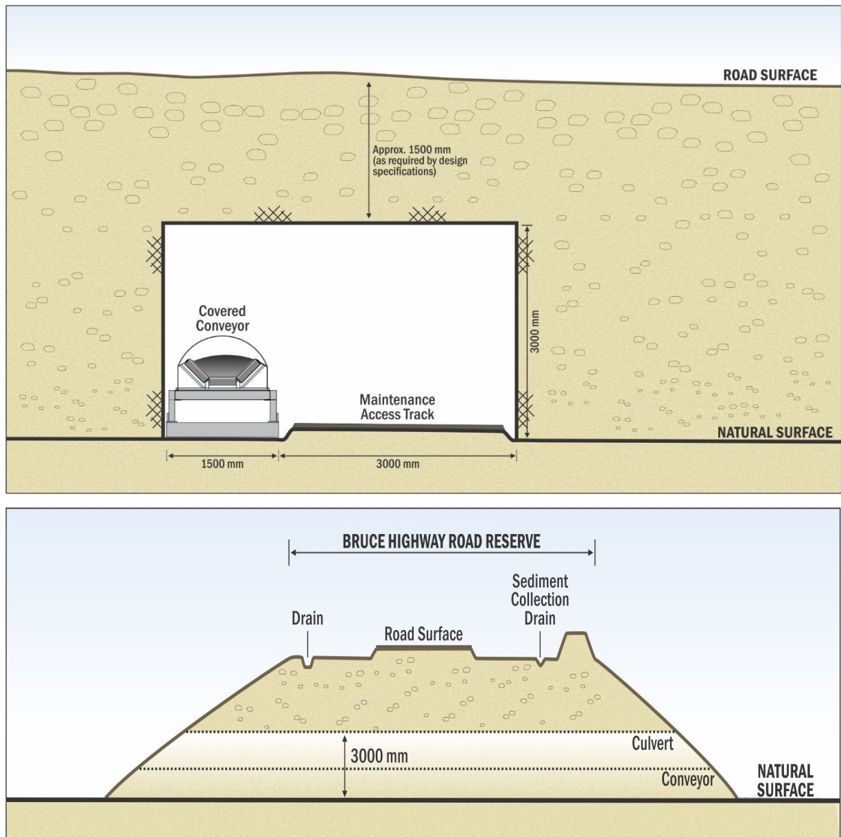
Figure 6-4: Indicative conveyor arrangement under the Bruce Highway
