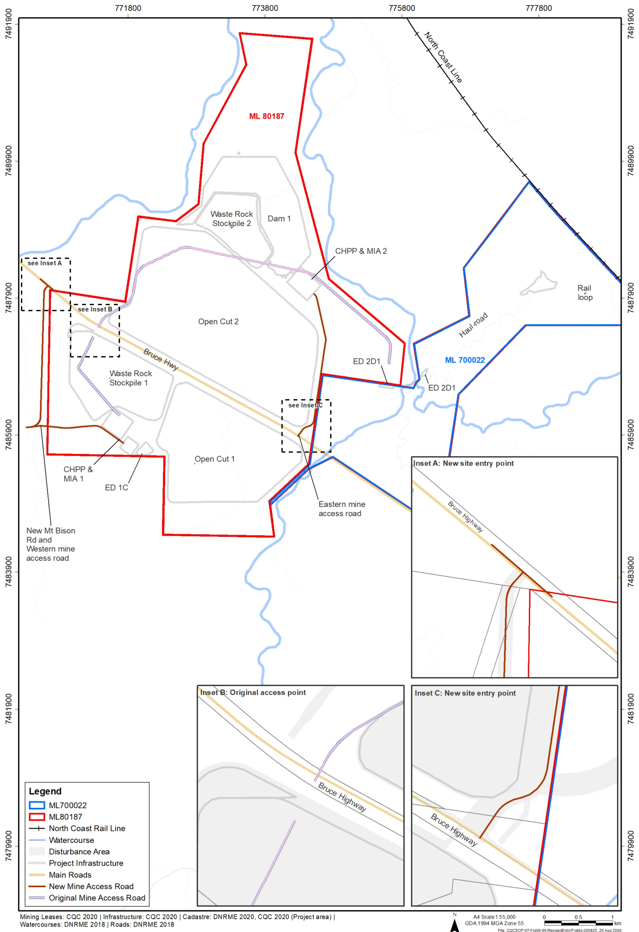
Figure 6-1: Revised eastern and western mine entry access points
